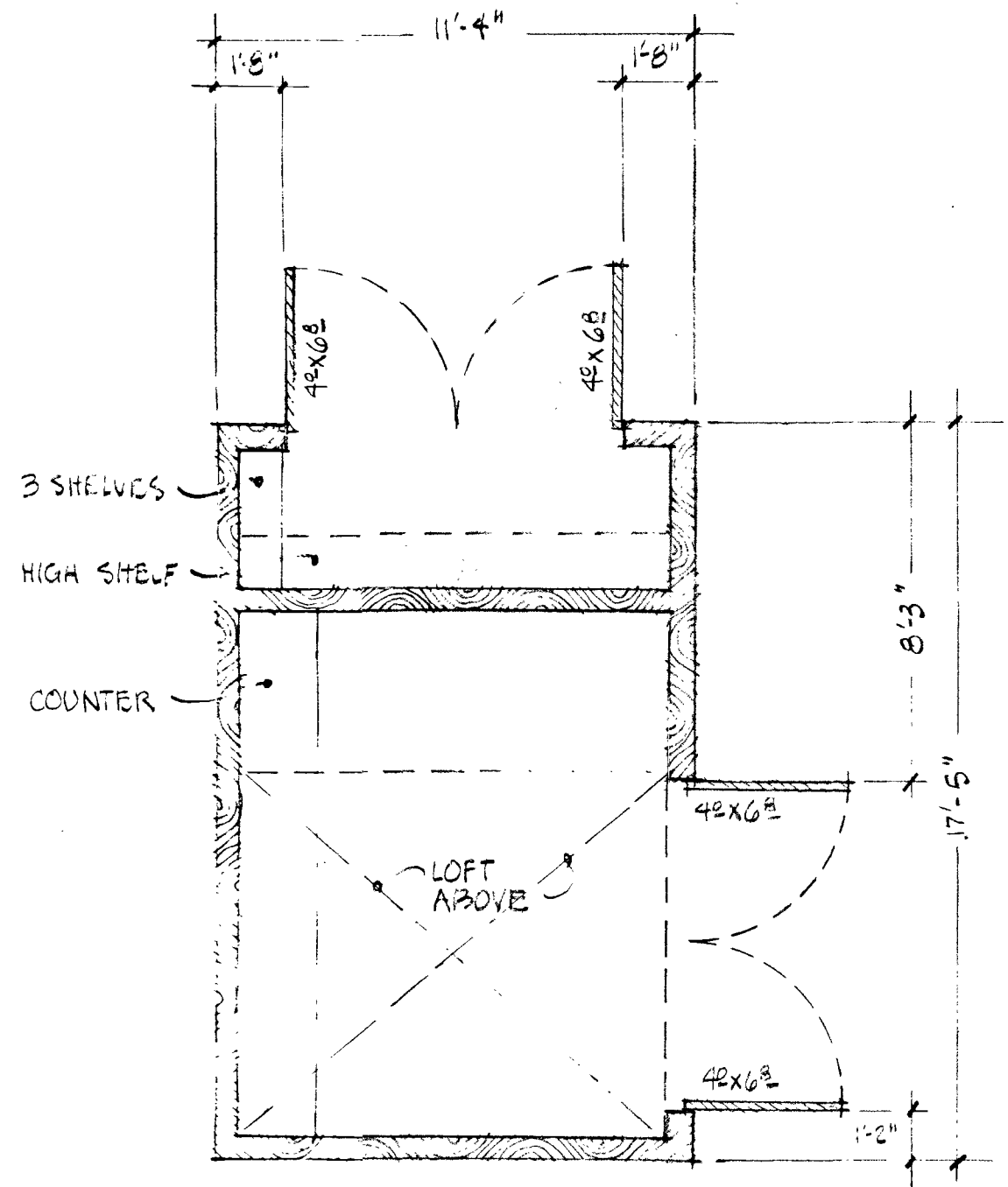
FLOOR PLAN / CARTER UTILITY BUILDING 1/4" = 1'-0" ← NORTH
