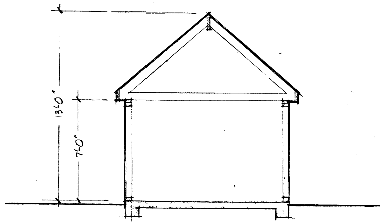
SECTION 1/4" = 1'-0"
